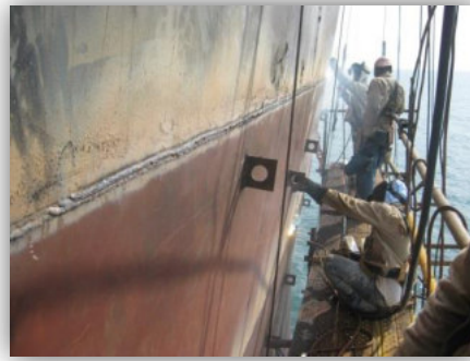
Steel Renewal
