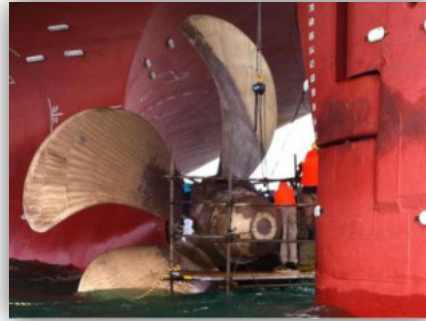
Propeller Repair
